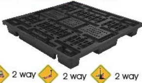
SEL 1111 MH Sello Nestable Pallet 1111 MH Size 1100x1100x130 mm.
